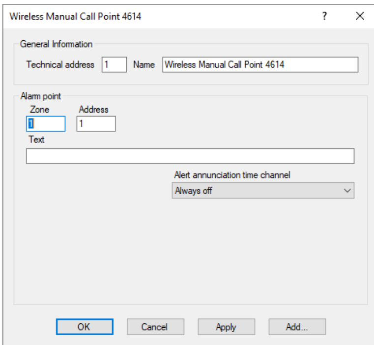
EBLWin dialog box "Wireless manual call point 4614."
