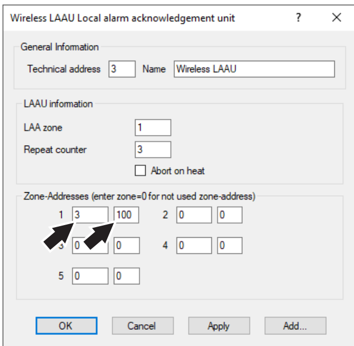
EBLWin dialog box "Wireless local alarm acknowledge unit 4645.
